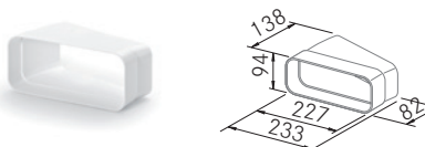
Flat Horizontal Bend Ducting 15°
