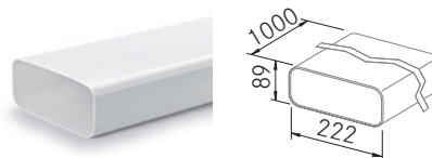
Flat Ducting Connector
