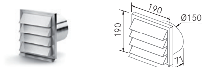
Exterior Exit Deflector Ø 150
