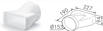
Flat Round Adapter
