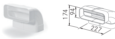
Horizontal 90° Elbow Flat
