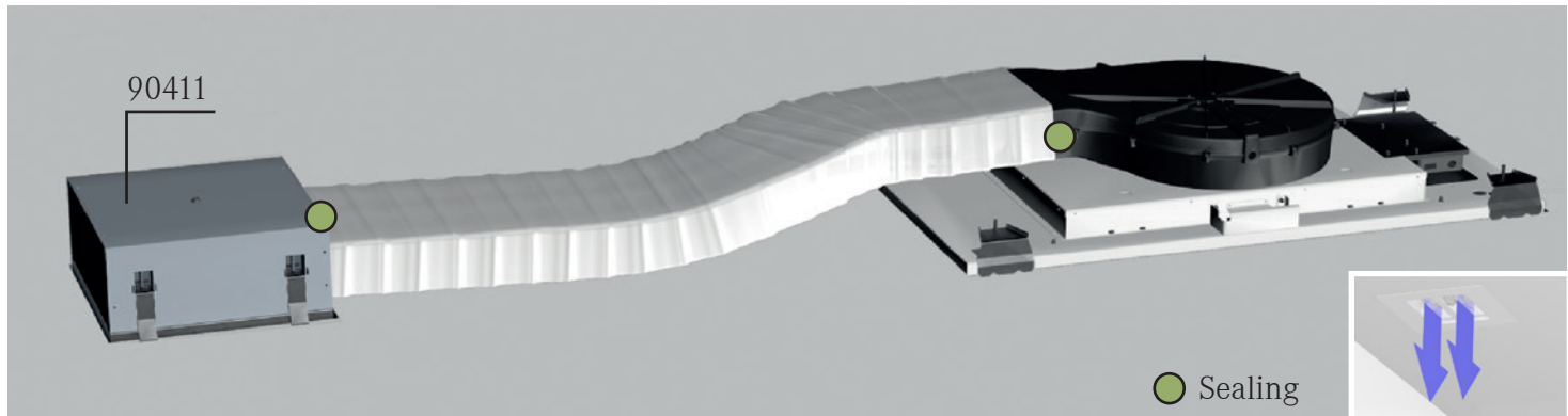
Example of installation of the H2 Filter system with 2-Motors Ceiling Hoods
